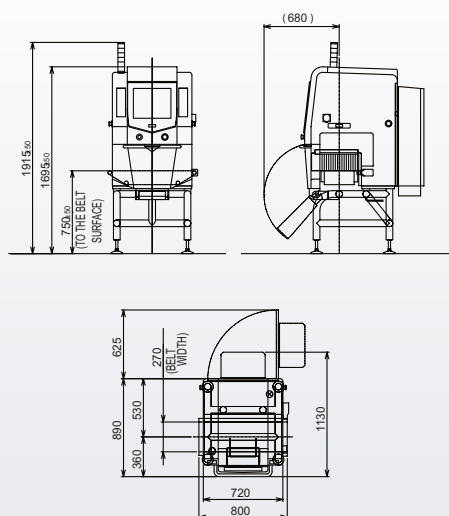
Dimensions - IX-G2-2427
