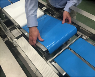
Quick-release belts
